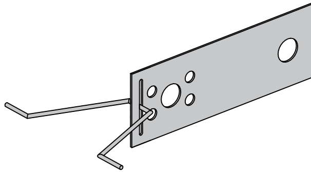
ICF WALL BRICK TIE
