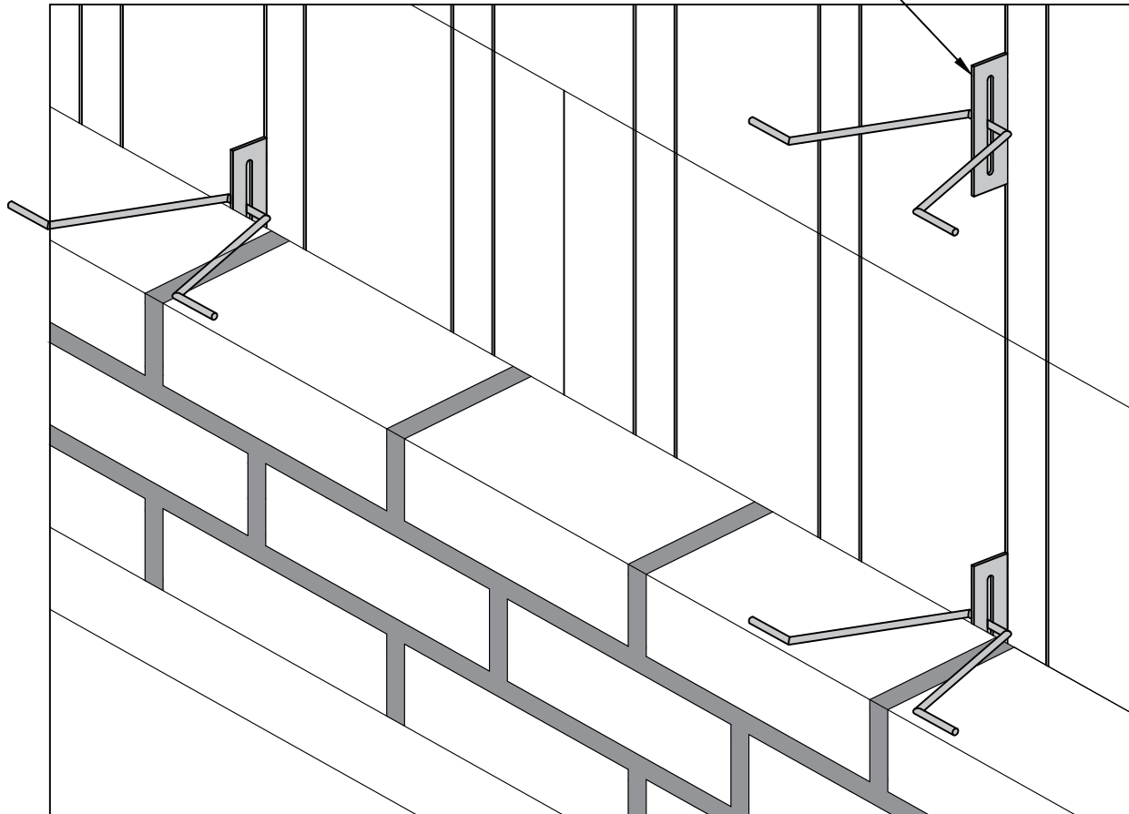
ICF WALL BRICK TIE
