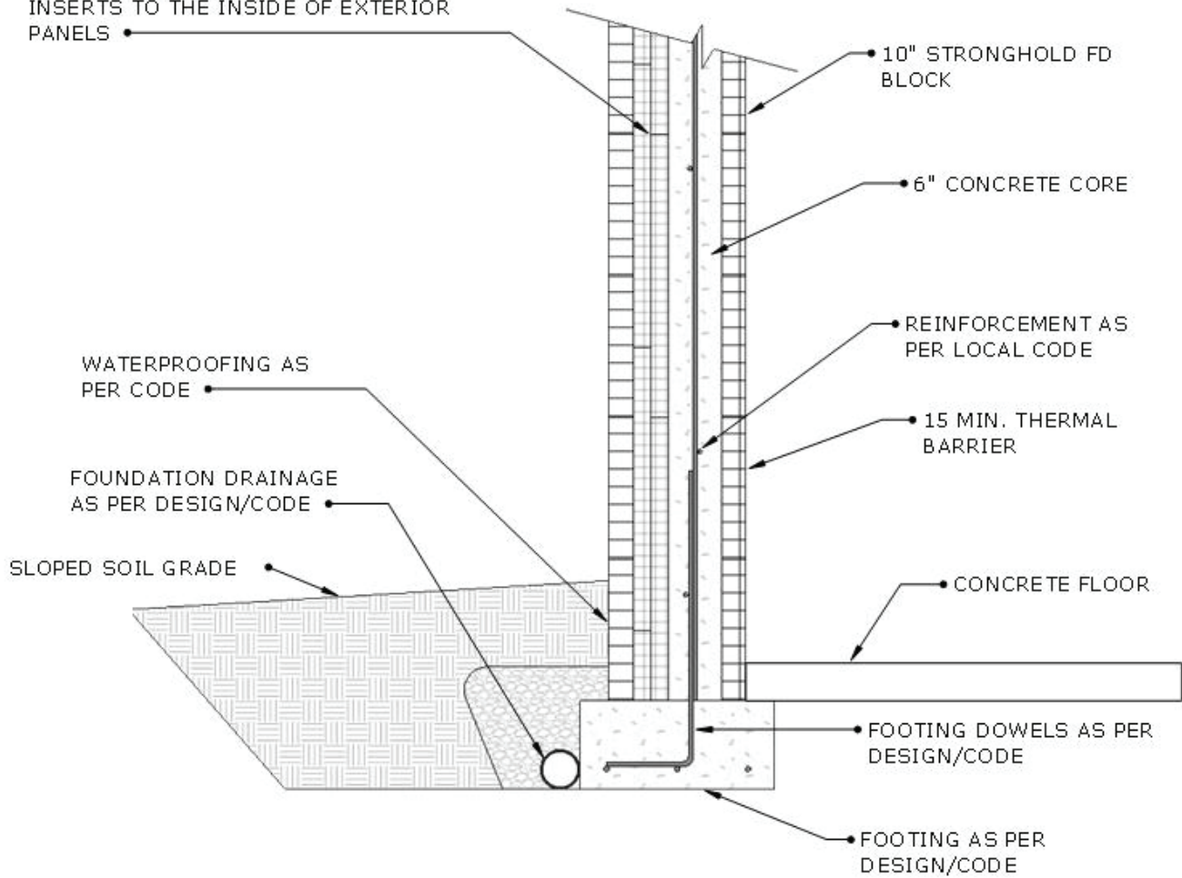
STRONGHOLD WALL SECTION WITH DOUBLE 2" EPS FOAM INSERTS
